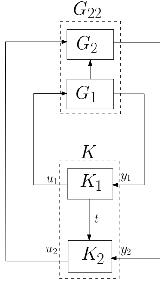
Figure 2.5 2-nest system with signal t transmitted from inner nest sub-controller K_1 to outer nest sub-controller K_2
