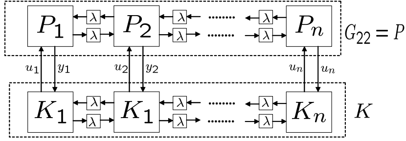
Figure 2.6 Banded structure system.
