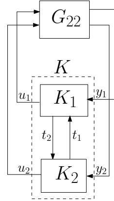
Figure 2.1 The G - K_1 - K_2 interconnection Figure 2.2 G_{22} - K_1 - K_2 interconnection
