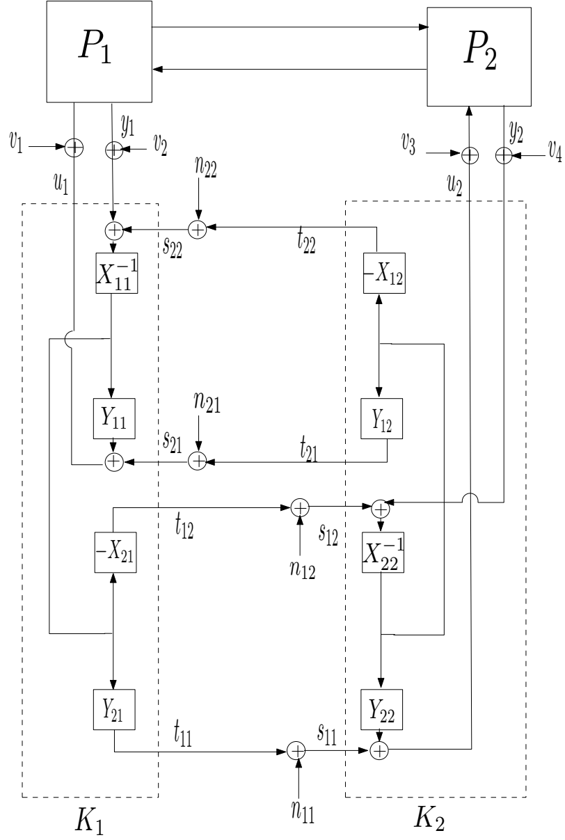
Figure 3.3 Right-coprime architecture
