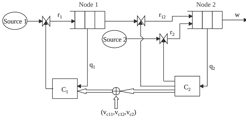
Figure 6.1 2-nodal ABR network with congestion control
