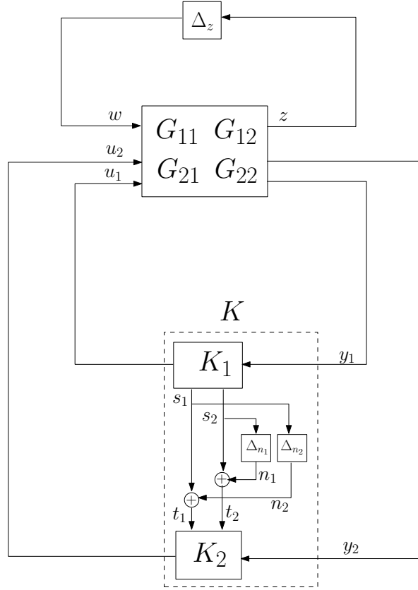
Figure 5.1 G - K nested system with noise modelled as multiplicative uncertainty
