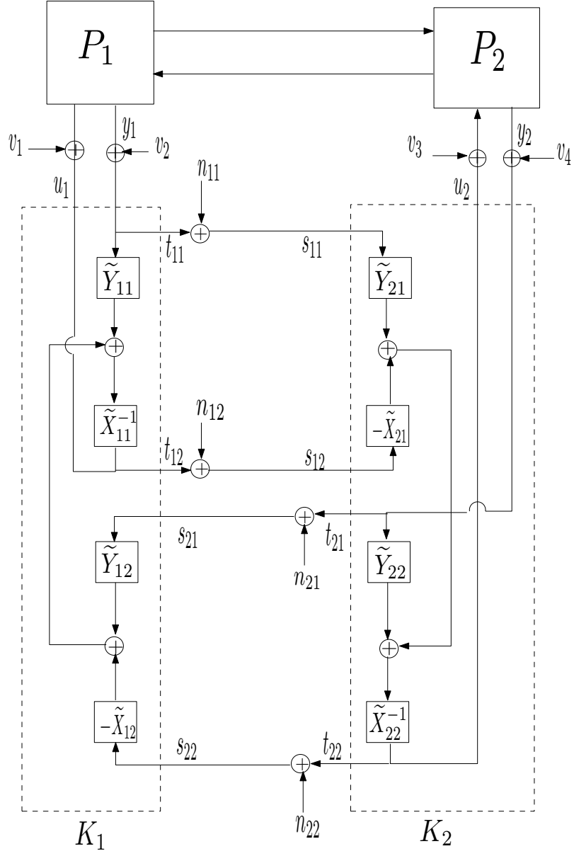
Figure 3.2 Left-coprime architecture
