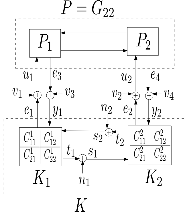
Figure 3.1 The controller with communication noise n_1 and n_2
