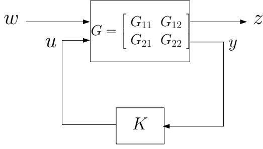
Figure 2.3 The G-K interconnection
