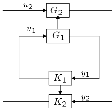
Figure 2.7 Nested structured system
