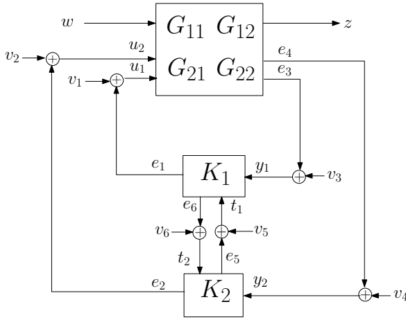
Figure 2.1 The G - K_1 - K_2 interconnection Figure 2.2 G_{22} - K_1 - K_2 interconnection
