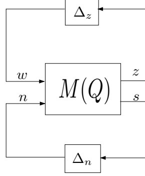
Figure 5.2 The M - \Delta configuration for two channel case shown in Figure 5.1
