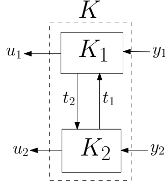
Figure A.1 Distributed implementation of K
