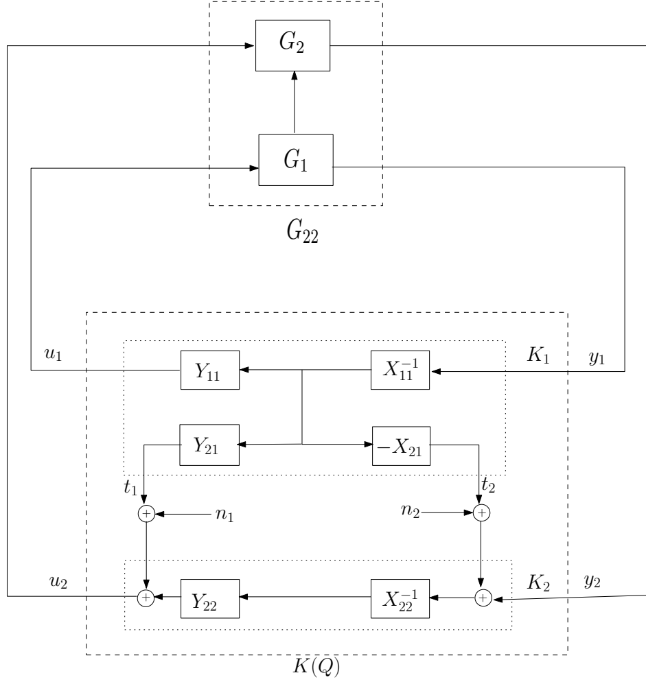
Figure 4.4 Right-coprime architecture for nested structure
