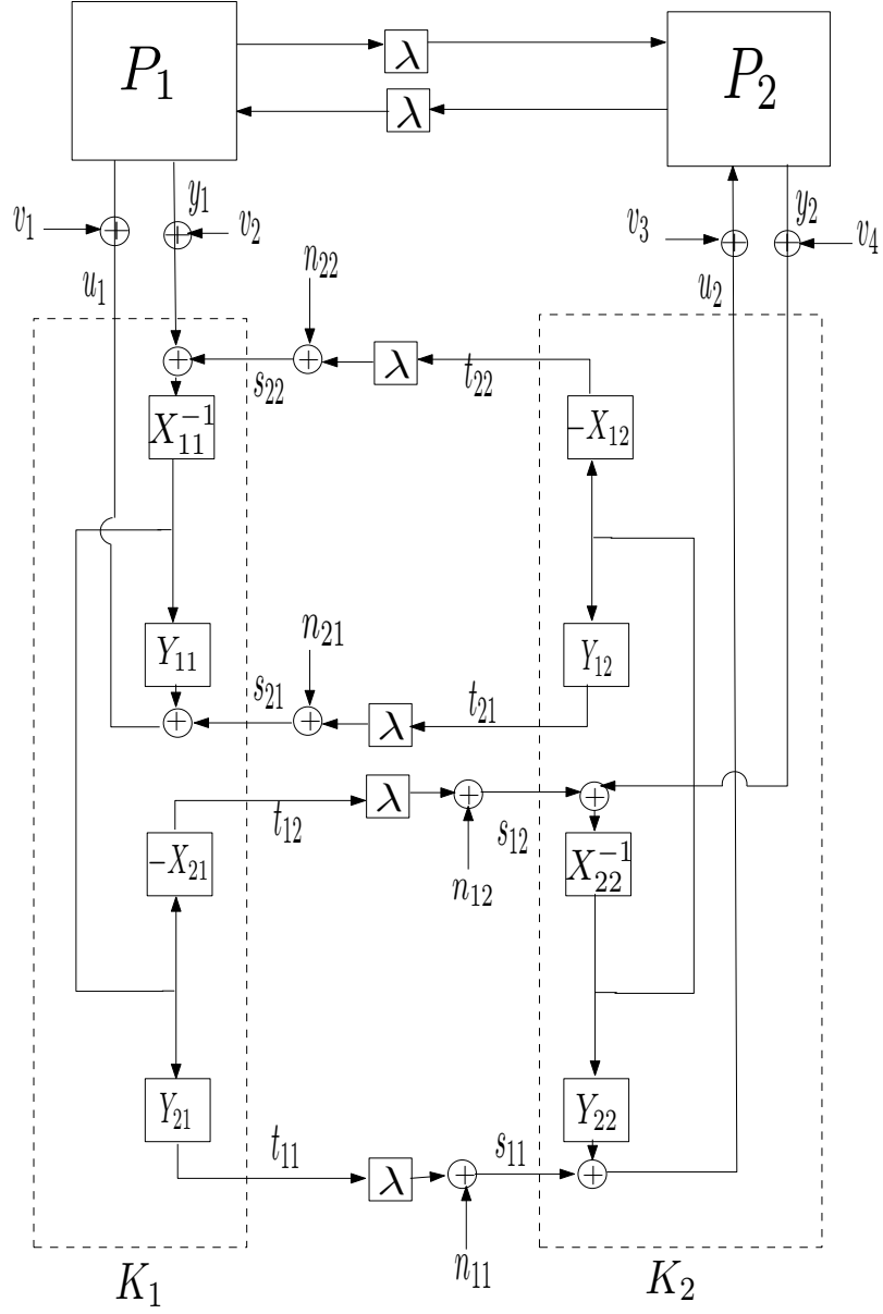
Figure 4.2 Right-coprime architecture for banded structure
