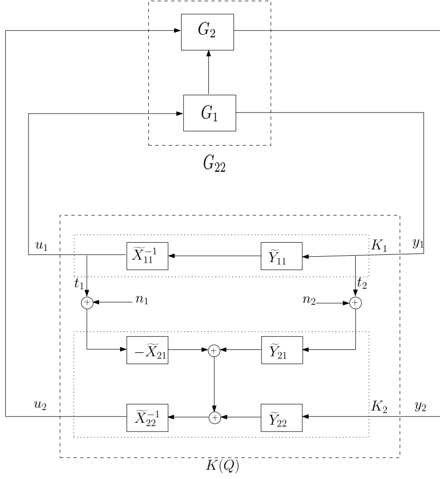
Figure 4.3 Left-coprime architecture for nested structure
