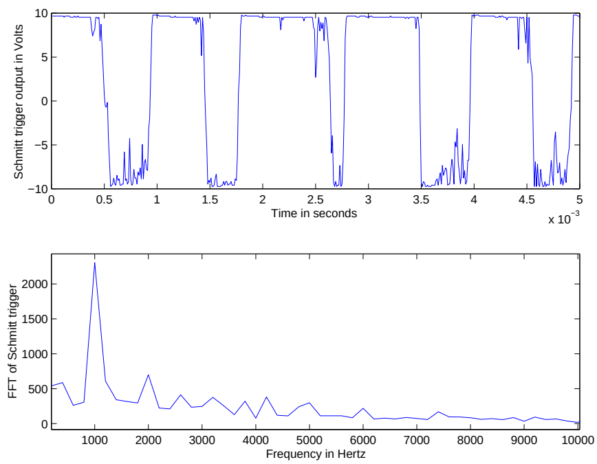
Figure 1.15 Experimental results on the Schmitt trigger
