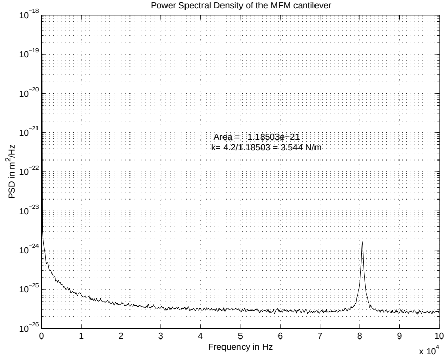
Figure 3.3 Experimentally observed PSD curve of the MFM cantilever
