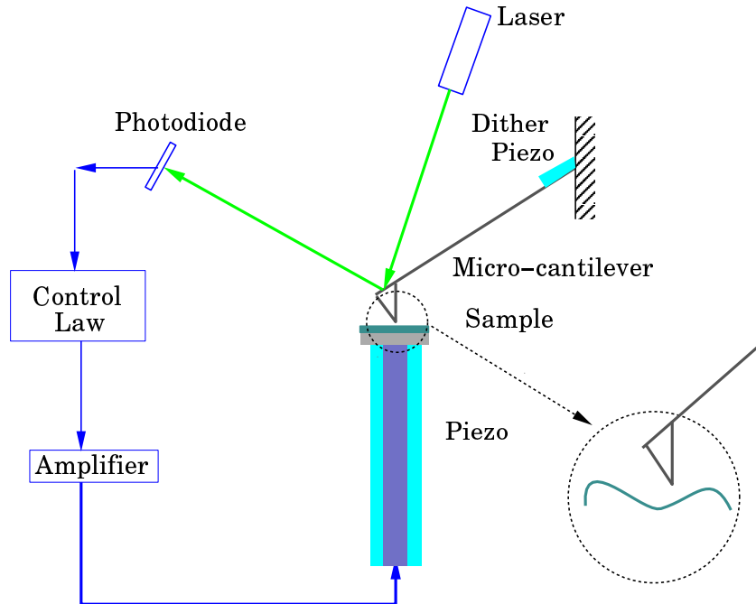
Figure 1.2 A schematic of the AFM
