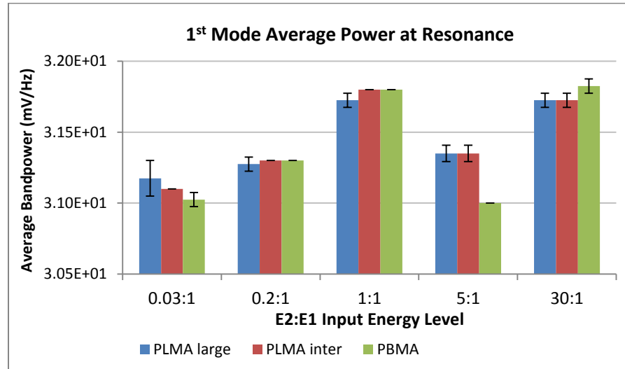
Figure 4.10: Average bandpower of the first mode at resonance frequency
