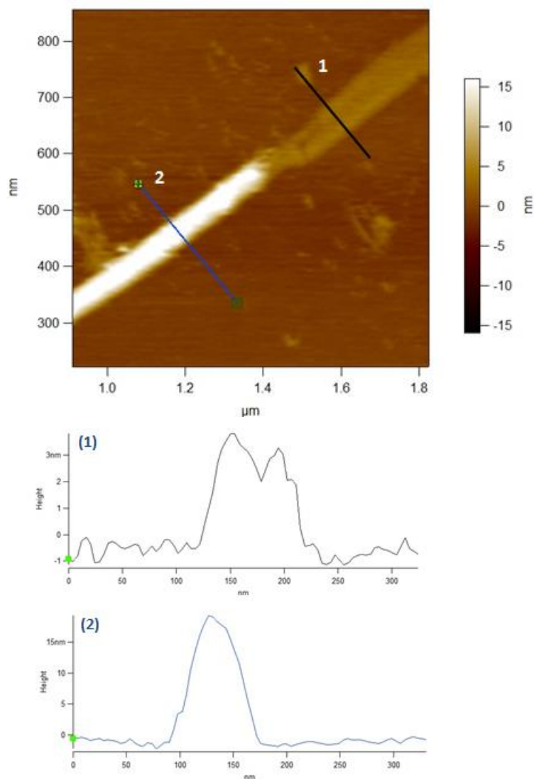
Figure 6.10: Topography (top) and cross-section profiles (bottom) showing the collapsed and non-collapsed regions of the microtubule strand. A collapsed portion and a structurally-intact portion of a microtubule strand are approximately 4 nm and 20 nm tall, respectively. The width of the taller microtubule segment is approximately 100nm, whereas the collapsed segment is wider. The collapse or flattening of the microtubule region might be due to the applied tip force during imaging.
