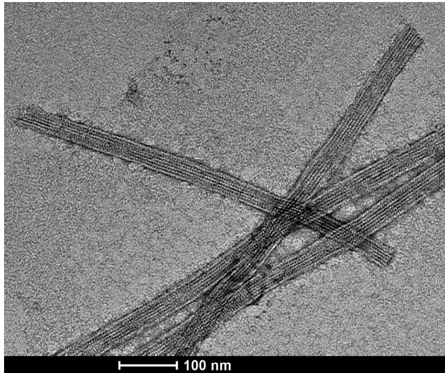
Figure 6.2: TEM image of multiple microtubules. Approximately 7 striations of protofilaments are visible for each microtubule. The width of the microtubule strand is approximately 50nm. The microtubule width is highly dependent on the sample preparation techniques (TEM image provided by Professor M. Gardner's research group at UMN)
