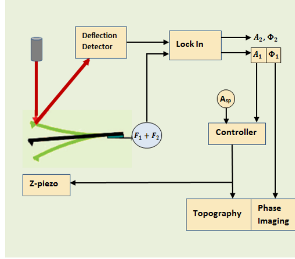
Figure 1.2: In the typical bimodal dynamic AFM operation, two external excitation signals, F_1 and F_2 , are added to drive the cantilever. The excitation signal is chosen near the resonant frequency of the first and second mode. This signal is fed back to the lock-in amplifiers, and the first and second mode signals are demodulated at the drive frequencies to obtain the amplitude and phase signals for each mode. The first mode amplitude signal is used as the feedback to the Z-piezo, whereas the second mode is exploited to obtain additional material property contrast. A_{sp} is the amplitude setpoint imaging parameter.
