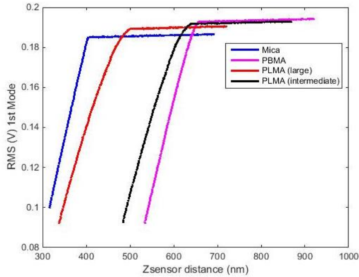
Figure 4.4: Estimated first mode RMS amplitude vs. Zsensor
