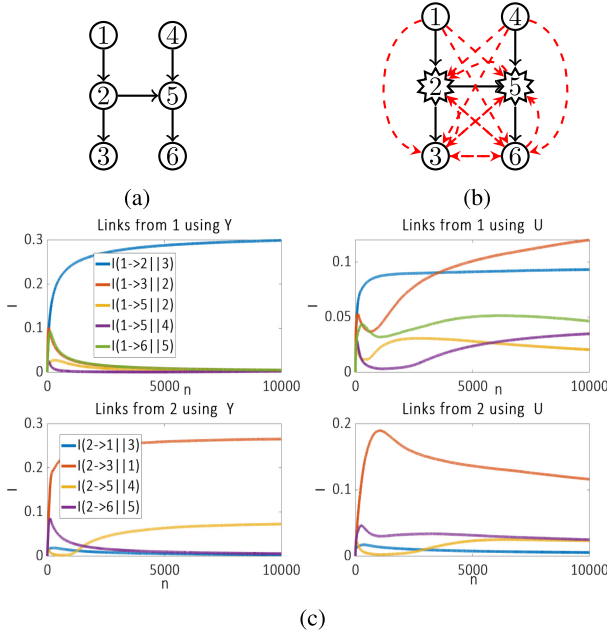
Fig. 6. (a) True generative graph. (b) Perturbed graph inferred. (c) DIR estimates to detect links from nodes 1 and 2 using ideal measurements Y and when there is corruption at nodes 2 and 5. The spurious links are shown in red and the true edges are shown in black. With cascaded perturbations, more spurious links are inferred.
