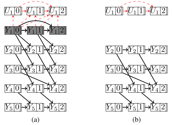
Fig. 3. (a) Perturbed DBN G'_Z for 3 time slices when node 1 is corrupt. Node 1 ideal stream, Y_1 , is shaded because it is not measured. (b) Causal relations between the measured data streams without hidden Y_1 . There are no direct causal connections between time-series U_1 and other time series nodes as there are no direct dynamic influences between them, and therefore, are not shown.
