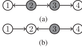
Fig. 1. When the trail connecting nodes 1 and 4 is active given Z . (a) Trail connecting 1 and 4 is active given Z = \{\} . (b) Trail connecting 1 and 4 is active given Z = \{2\} .
