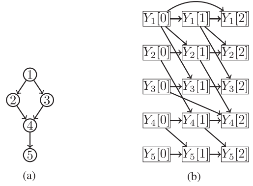
Fig. 2. (a) Generative graph and (b) its associated DBN for 3 time slices.
