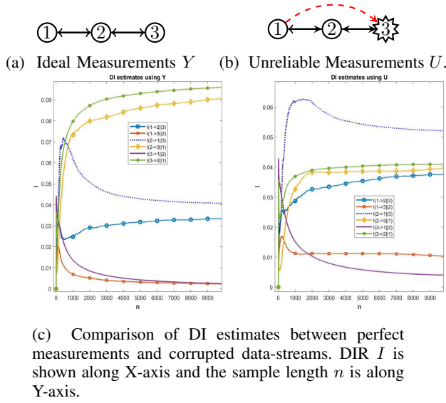
Fig. 2: Directed Information estimates: Note that only I(y_3 \rightarrow y_1|y_2) and I(y_1 \rightarrow y_3|y_2) keeps decreasing and asymptotically reaches zero. On the other hand, there is a rise in I(u_1 \rightarrow u_3|u_2) and it plateaus as sample length grows while I(u_3 \rightarrow u_1|u_2) continues to decrease. I(u_2 \rightarrow u_3|u_1) shoots and plateaus at an increased value compared to I(y_2 \rightarrow y_3|y_1) while other DI estimates continue to increase. We therefore infer the perturbed graph in Fig. 2b).
