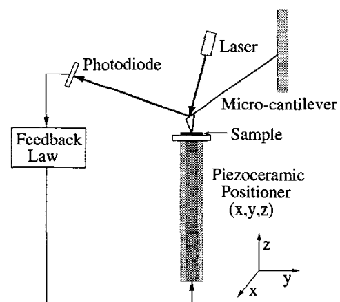
Figure 1. Configuration of a prototypical AFM.
