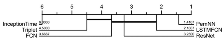
Figure 4. Critical difference diagram of different deep learning models across the simulated and experimental testing sets of all protein molecules based on average accuracies. The most accurate model is assigned a rank of 1, with a thick horizontal line representing a group of classifiers that do not exhibit statistically significant differences in accuracy.
