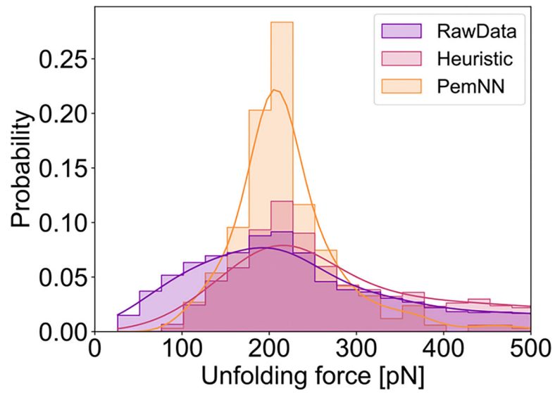
Figure 7. Application to SMFS data analysis of Titin I27O: RawData as the Baseline Method, Heuristic as non-machine learning method, and PemNN as the our proposed model.
