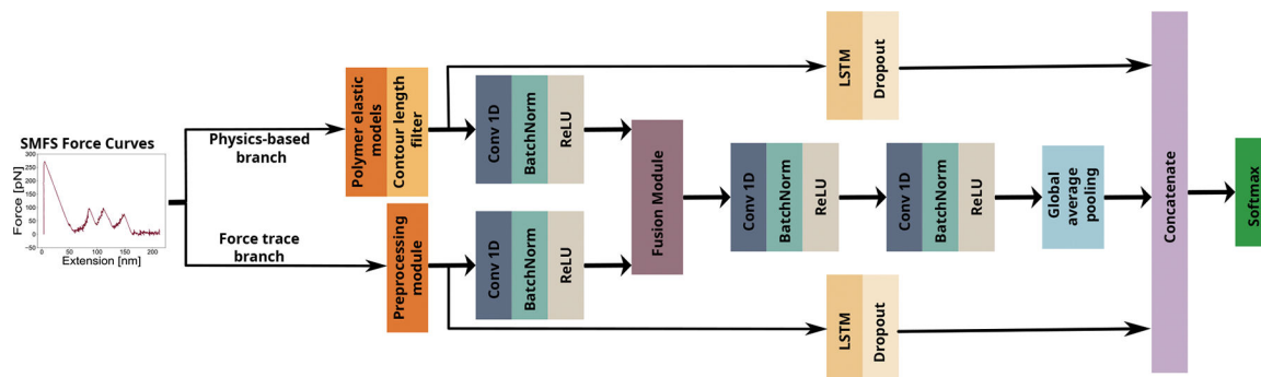
Figure 2. The overall architecture of the Polymer Elastic Models Neural Networks (PemNN) comprises a physics-based branch and a force trace branch, illustrated with the early fusion approach (the late fusion approach is shown in Figure 8 in the Appendix).
